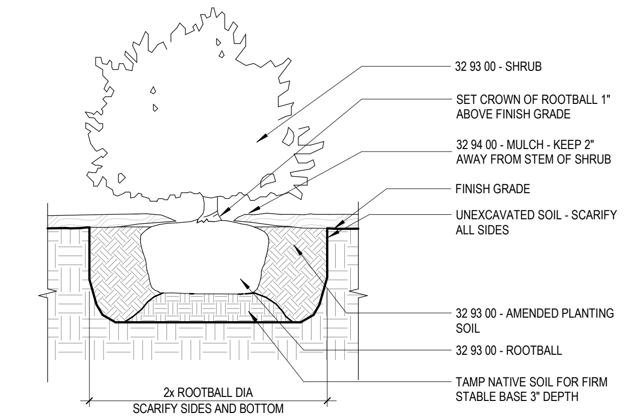
1 CONTAINER/B & B SHRUB 1" = 1'-0"
